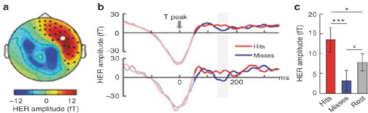
Figure 4: Neural events locked to heartbeats before stimulus onset predict the detection of a faint visual grating in the posterior right inferior parietal lobule and the ventral anterior cingulate cortex [69].
